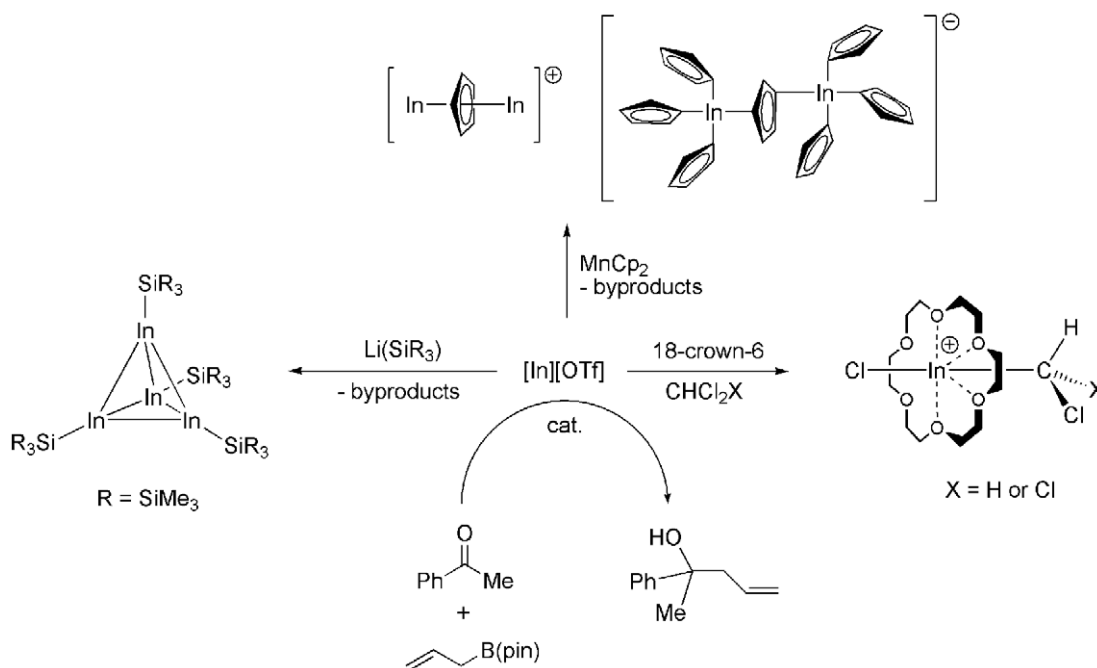
Scheme 2. Some of the reported organometallic chemistry of InOTf.
